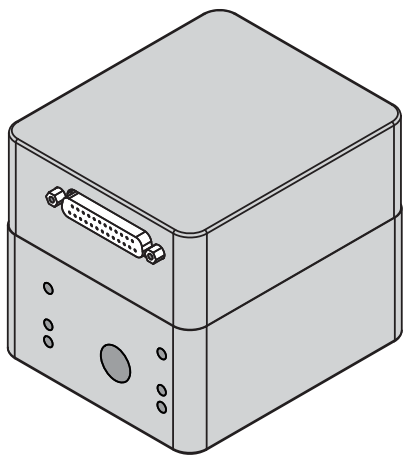
DIGITAL POWER IN (25-pin female D-SUB connector)
